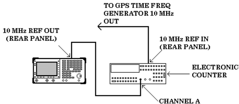
Figure 1. Frequency reference setup.
